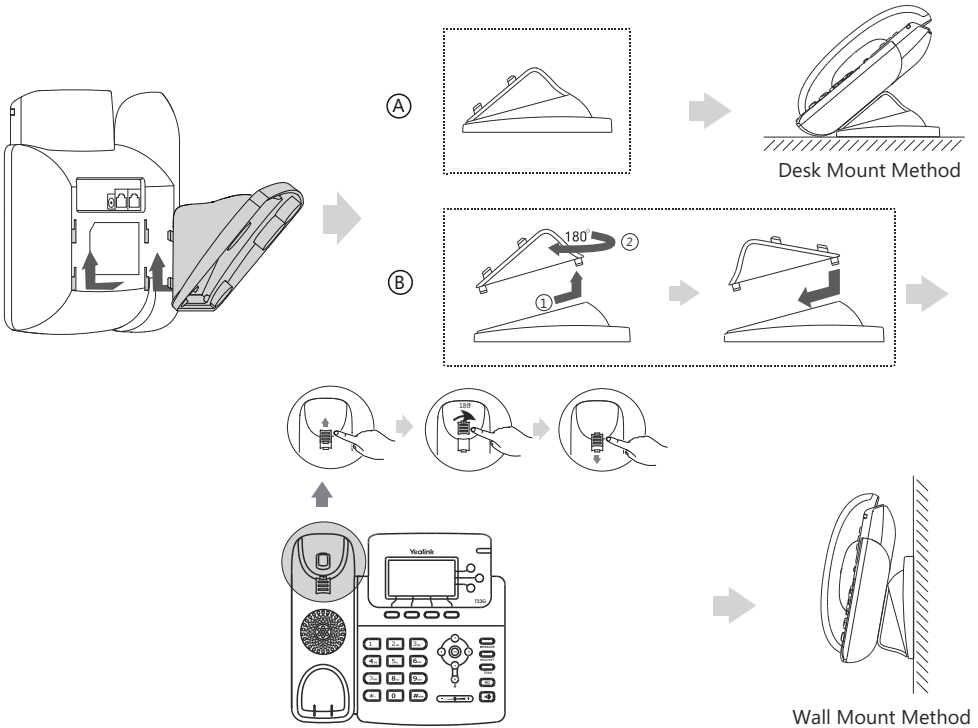
Wall Mount Method
